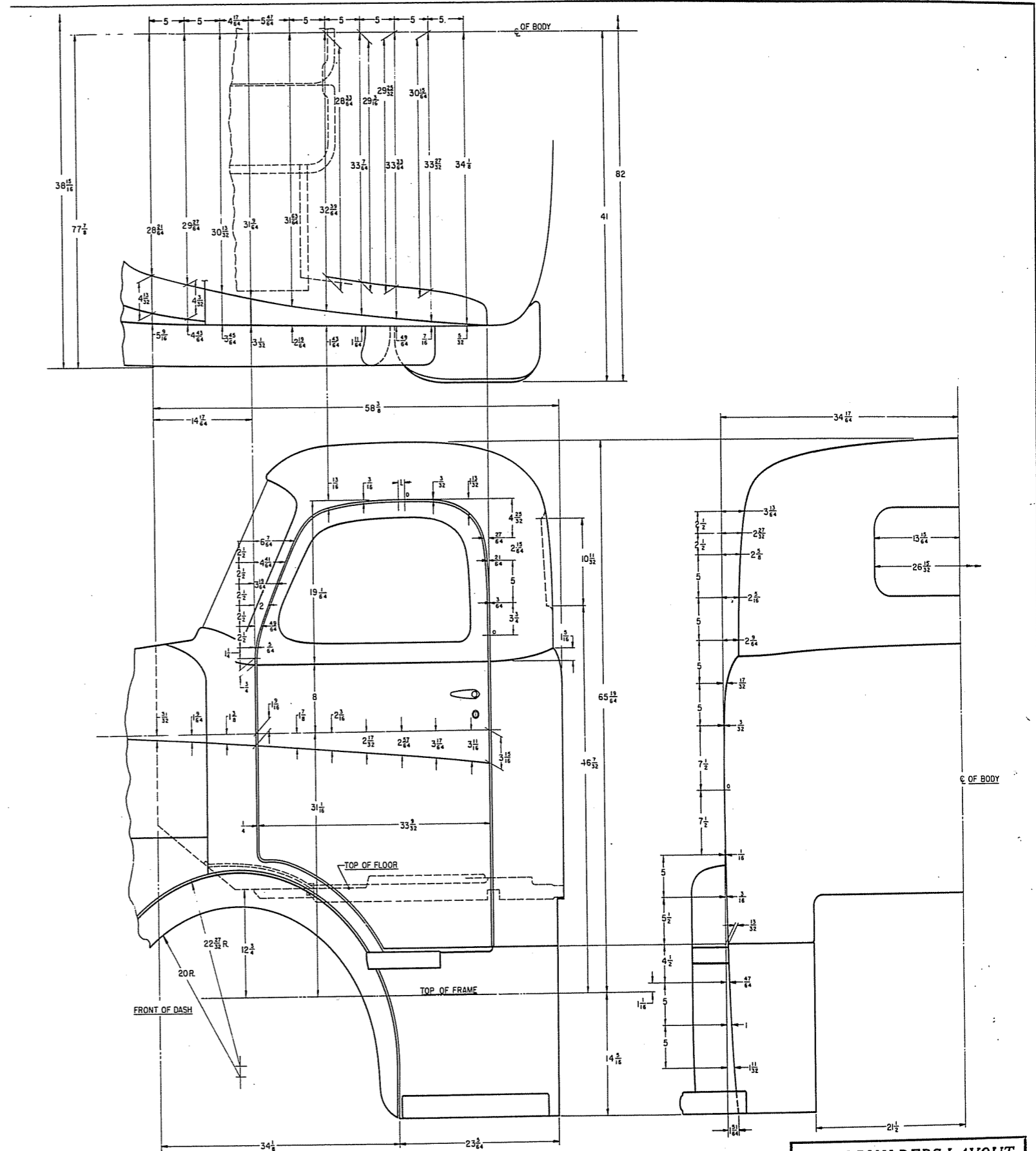
BODY BUILDERS LAYOUT CAB-C.O.E.
