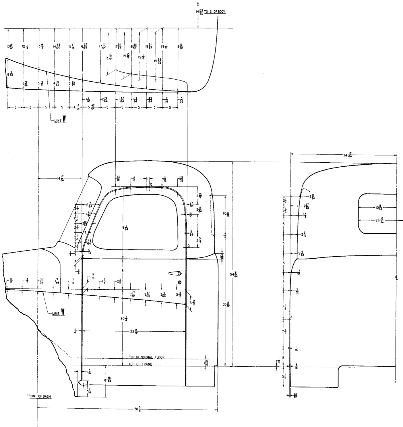
BODY BUILDERS LAYOUT CAB-CONVENTIONAL (EXCEPT POWER WAGON)
